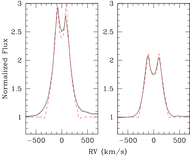
Fig. 13. Fits of the H \alpha line of HD 60 848 as observed in May 2000 ( left ) and the winter season 2013–2014 ( right ) with our disk model. The model is shown by the dashed line. The corresponding model parameters are given in Table 2. The failure to reproduce the line wings is probably because our synthetic models neglect electron scattering.
