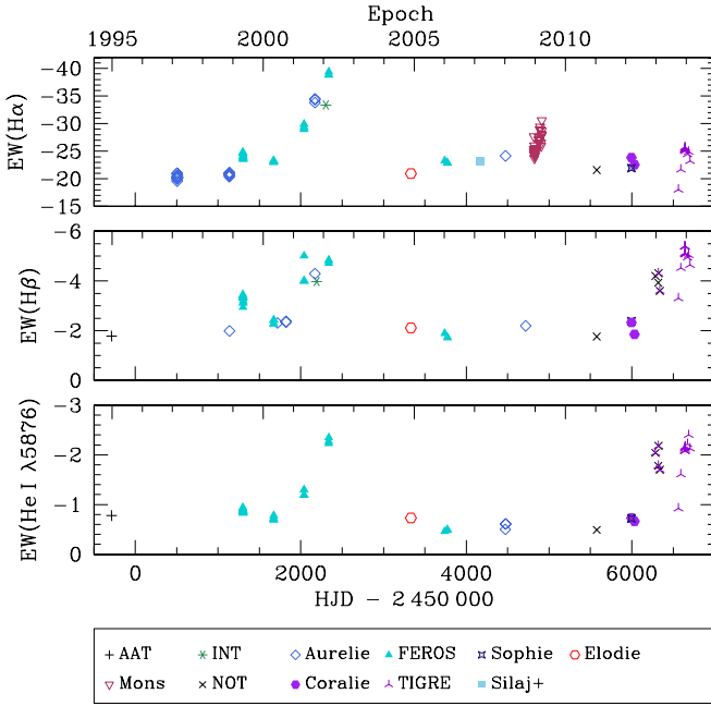
Fig. 7. Same as Fig. 3, but for HD 45314. Typical uncertainties on the EWs are 0.50, 0.25, and 0.20 Å for the H \alpha , H \beta , and He I \lambda 5876 lines respectively. We have also included the EW(H \alpha ) measurement of Silaj et al. (2010). The second Coralie spectrum was taken simultaneously with the XMM-Newton observation discussed by Rauw et al. (2013).
